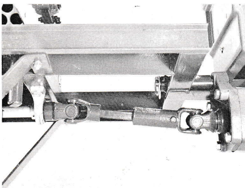
PTO shaft drive from tractor to shredder.
