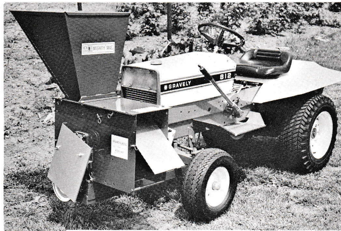
Model 9-G for Gravely 4 wheel tractors
